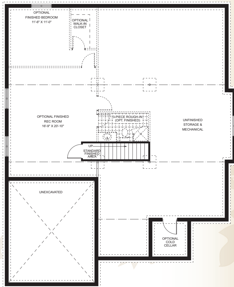
BASEMENT PLAN
